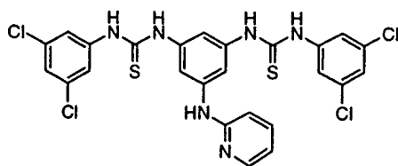
Compound # 13
